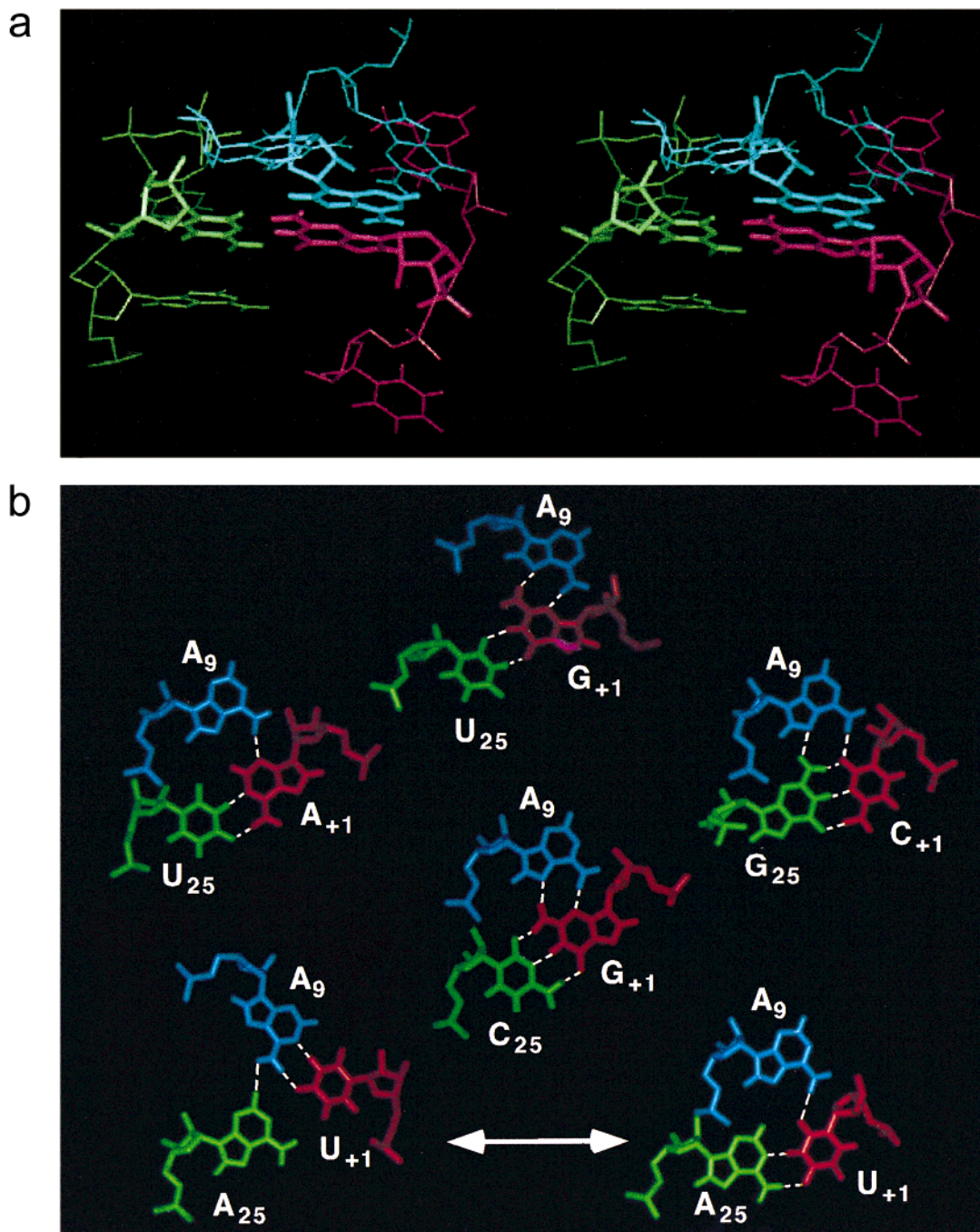
FIGURE 4: Molecular model of the A 9 •G +1 •C 25 triplet. (a) Stereoview showing the proposed base triple interaction involving G +1 (red) and its partners A 9 (blue) and C 25 (green). The nucleotides immediately 5' and 3' of the triplet also are shown (thinner lines). (b) Secondary structure of the proposed base triple. Compensatory variants of the triplet analyzed in this work are also indicated. The potential formation of a Watson-Crick base pair between U +1 and A 9 in the internal loop A may impair triplet formation and is consistent with the low level of restoration of cleavage activity of that combination (bottom).
