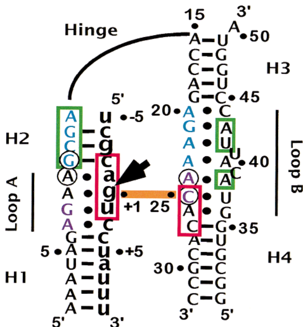
FIGURE 1: Secondary structure of the hairpin ribozyme-substrate complex. Interactions within internal loops A and B are as described previously (7, 8). Red and green rectangles indicate pairs of areas of the ribose-phosphate backbone protected upon domain docking and which are proposed to interact in the docked complex (10). Blue and lilac nucleotides indicate pairs of regions of the ribozyme that have been photochemically cross-linked (11). The circled nucleotides indicate the positions of the 2'-hydroxyl groups implicated in docking (22) and proposed to be involved in the formation of a ribose zipper between the two domains (9). The positions of nucleotides involved in the proposed Watson-Crick base pair ( G_{+1} and C_{25} ) are indicated by an orange line, and the cleavage/ligation site is indicated by a black arrow. The four helical segments are numbered H1-H4. Substrate is represented in lowercase letters.
